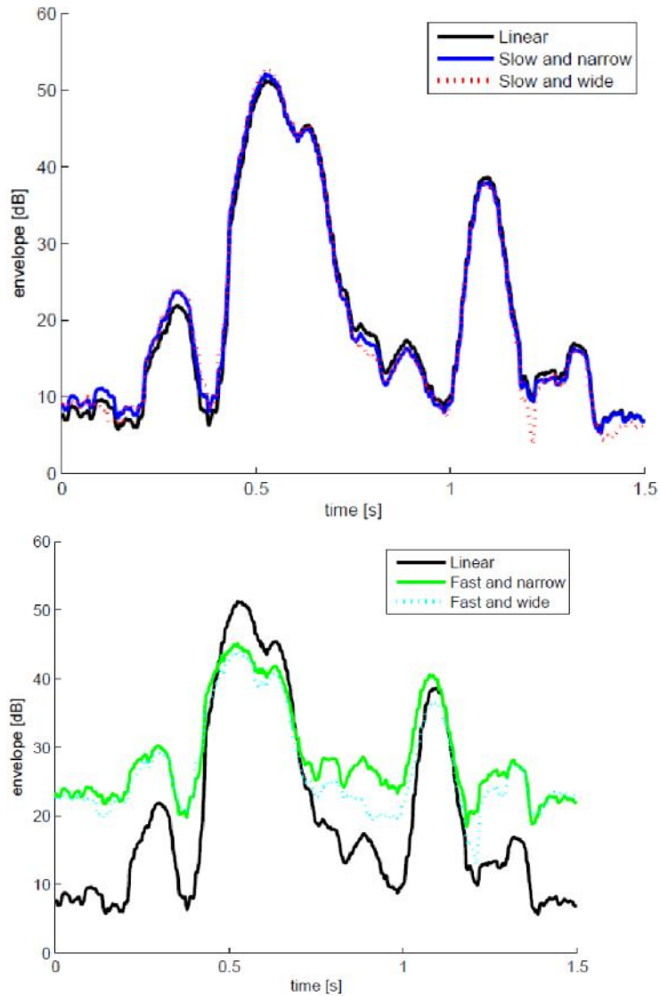
Figures 1a-b. Output envelope of a simulated 1000 Hz auditory filter generated from the Danish sentence “Nu kan en ny jagt begynde” (translation: “Now a new hunt can begin”) using slow-acting compression with wide (3-channel) and narrow (15-channel) frequency bandwidths (Figure 1a), and fast-acting compression with wide and narrow frequency bandwidths (Figure 1b). Linear processing is shown in black.
